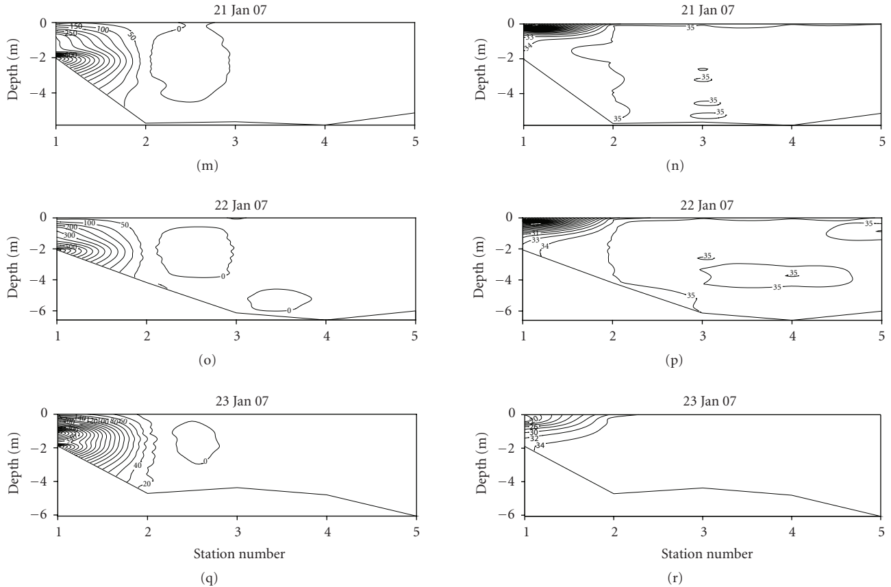
FIGURE 6: Snapshots at daily intervals of the two-dimensional distribution along the channel of salinity and SSC at Ngerdorch from CTD casts. The bottom line indicates the sea floor.
