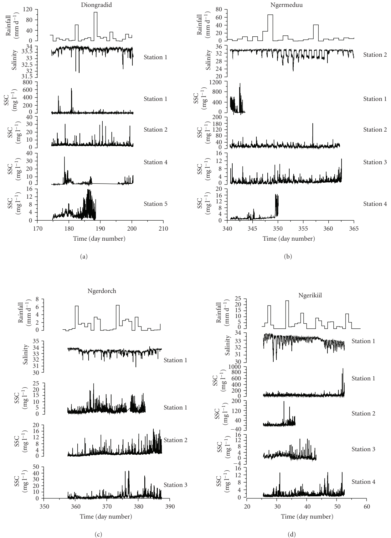
FIGURE 3: Time-series plot of rainfall, salinity and SSC at (a) Diongradid bay, (b) Ngermeduu bay, (c) Ngerdorch bay, (d) Ngerikiil bay.
