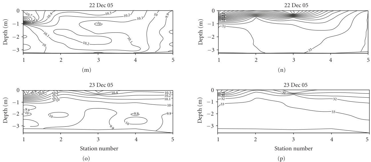
FIGURE 5: Snapshots at daily intervals of the two-dimensional distribution along the channel of salinity and SSC at Ngermeduu from CTD casts. The bottom line indicates the sea floor.
